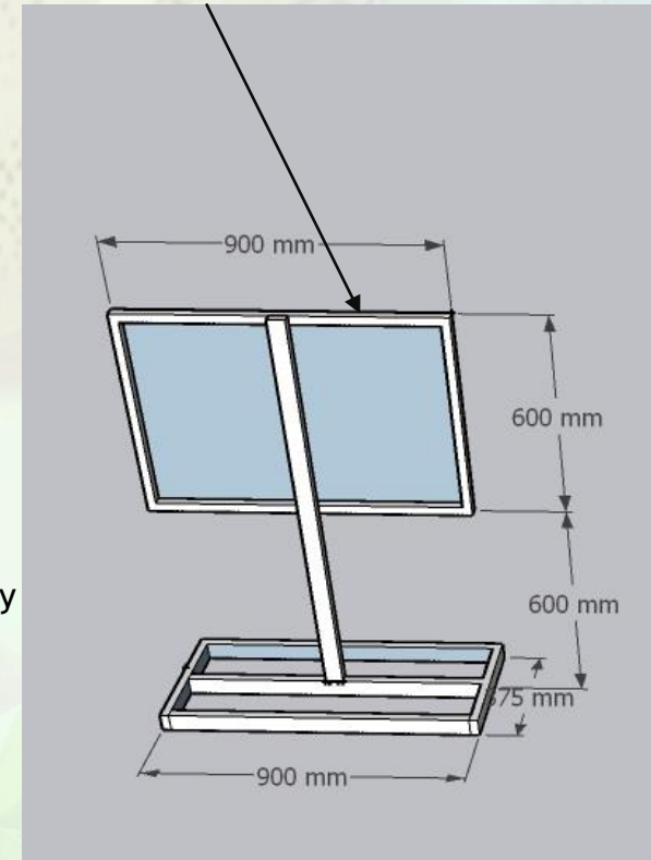
BACK SIGNAGE PANEL TYPE E
