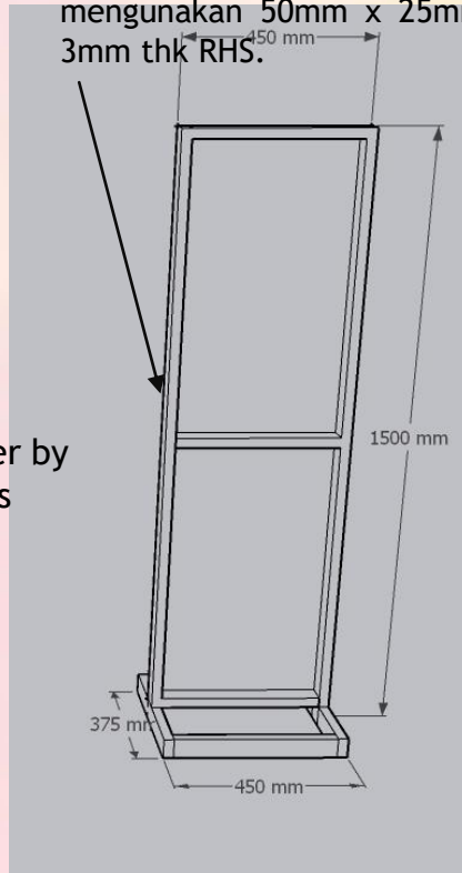
BACK SIGNAGE PANEL TYPE D
