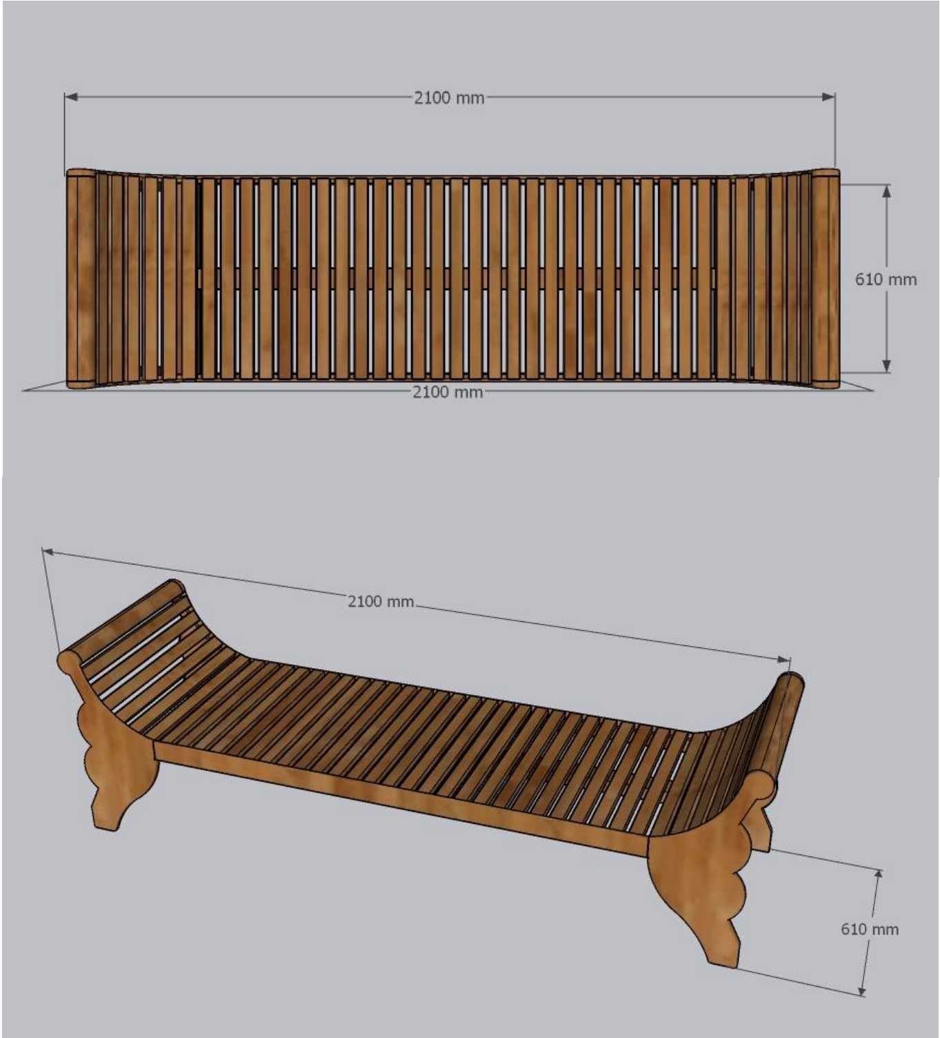
BANGKU TYPE B
