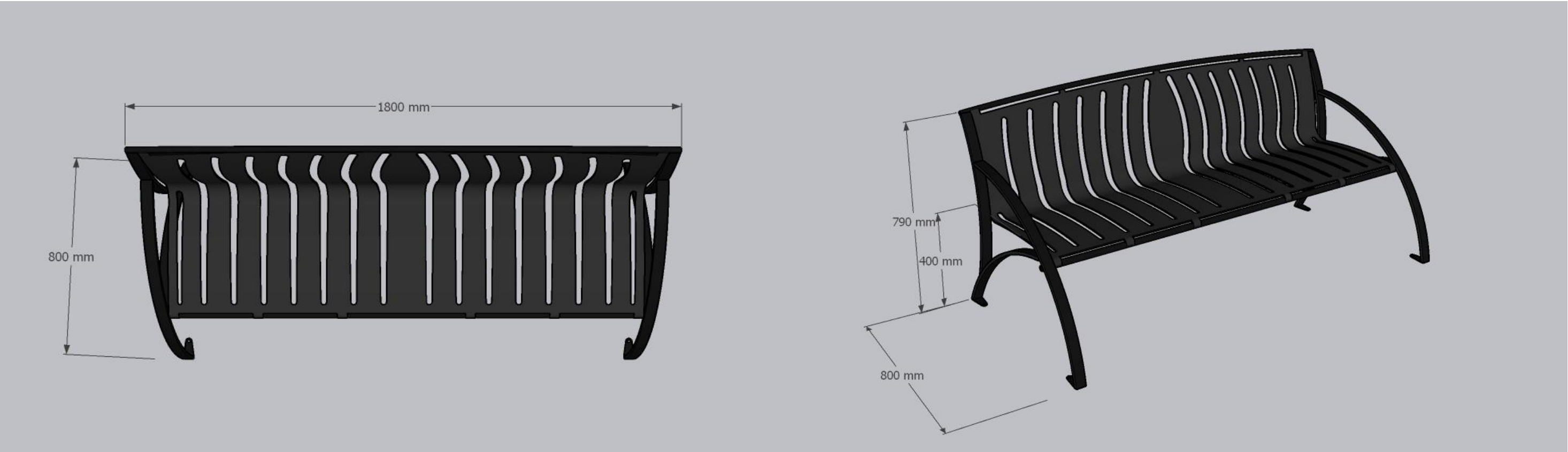
BANGKU TYPE C
