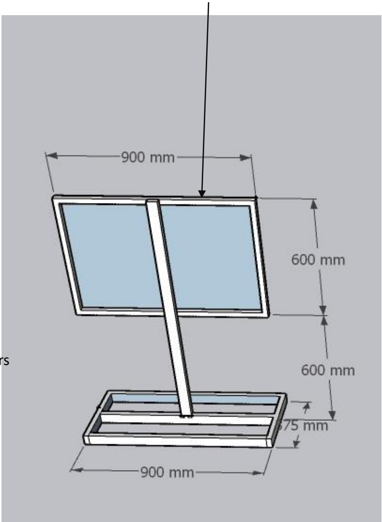
BACK SIGNAGE PANEL TYPE E
