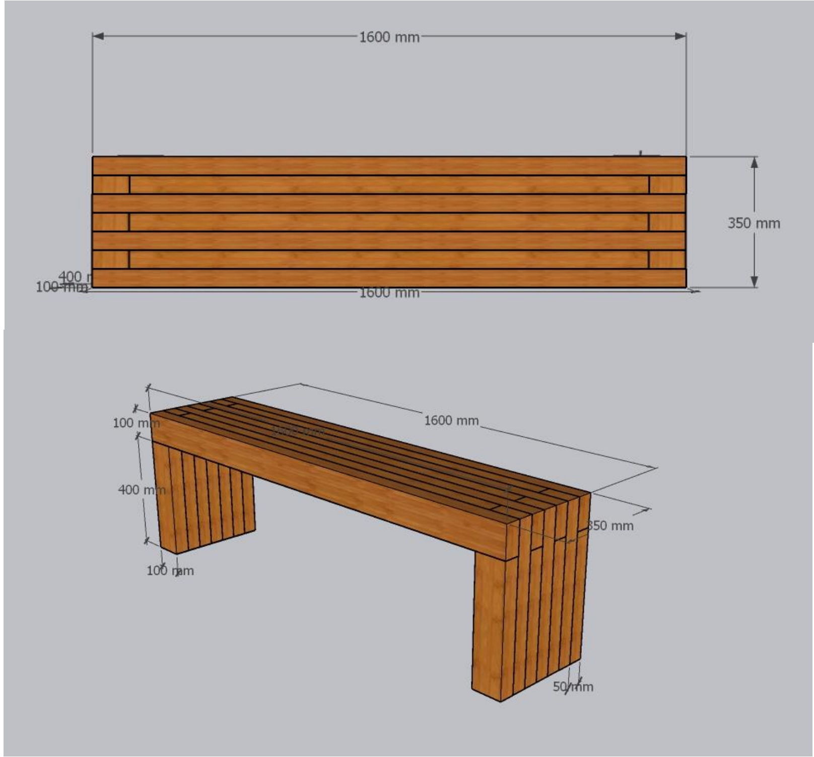
BANGKU TYPE A
