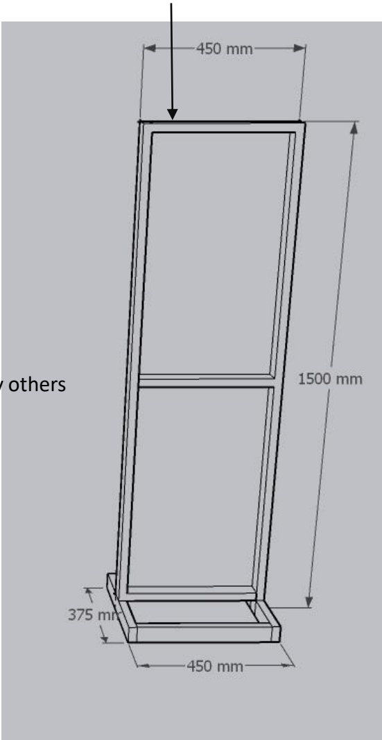
BACK SIGNAGE PANEL TYPE D
